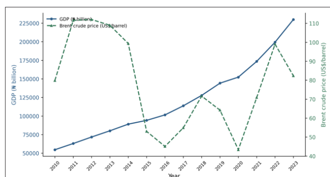
Figure 1: GDP and Brent crude oil price trend, 2010–2023 Author's Output (2026), based on data described in Section 5.2.
