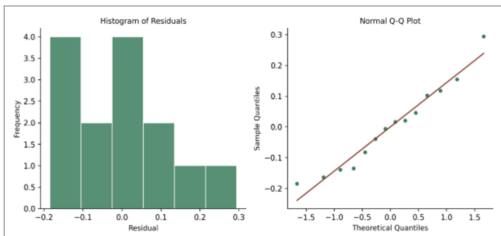
Figure 4: Residual diagnostics: histogram and normal quantile-quantile plot Author's Output (2026).
