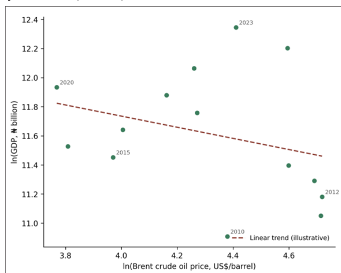
Figure 2: Scatter plot of \ln(\text{Brent crude oil price}) against \ln(\text{GDP}) Author's Output (2026).
